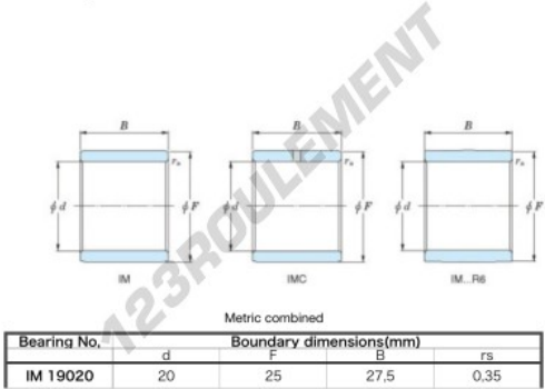
Boundary dimensions
